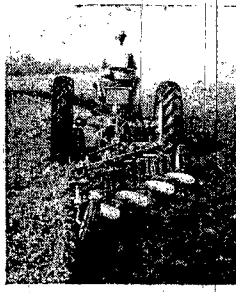
The new Model "70" has the power to handle four 14-inch plow bottoms (above) in most conditions, five 14's (far right) in many soils ... a 14-foot tandem disk harrow ... 20-foot disk tiller and many similar big-capacity tools.
